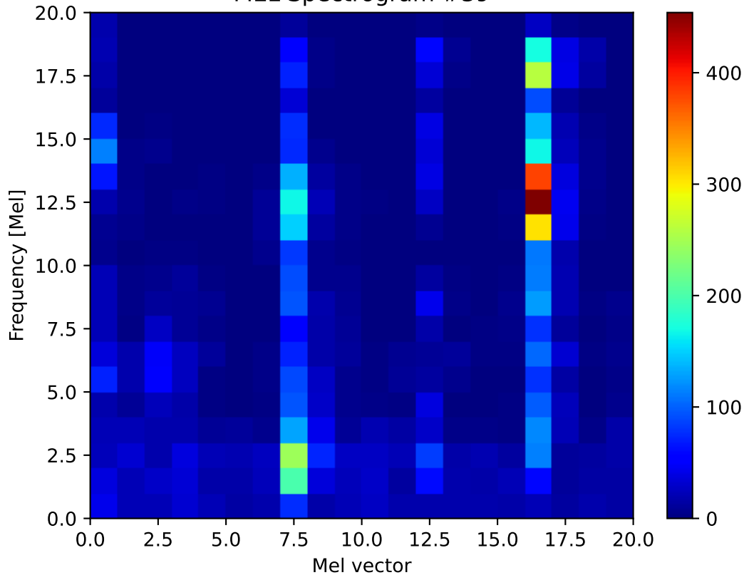
MEL Spectrogram #39
